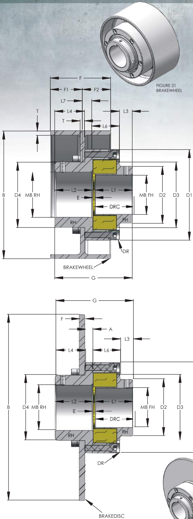
FIGURE 22 BRAKEDISC
